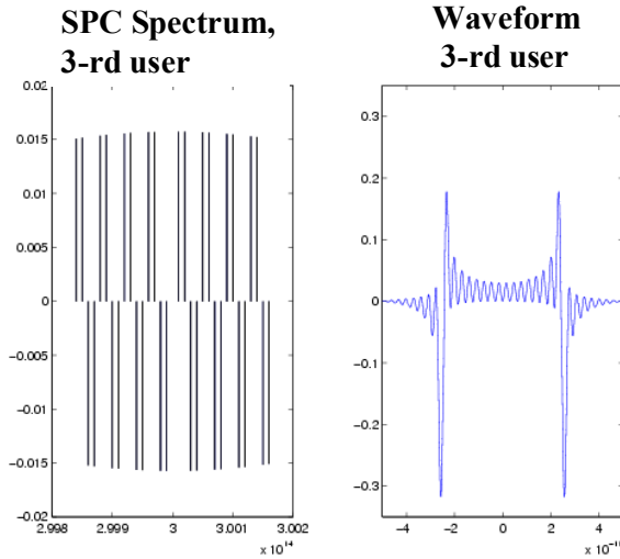
Fig.2 SPC Spectrum and Waveform
