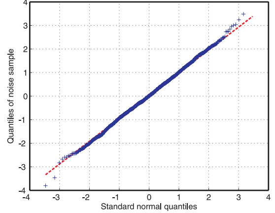
Fig. 7. Quantile-quantile plot comparing a real-valued standard normal distribution with measured samples of our RF-chain implementation.
