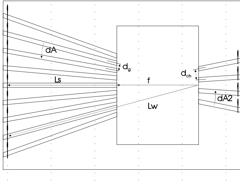
Figure 4. Schematic representation of the simulation configuration for the output star coupler
