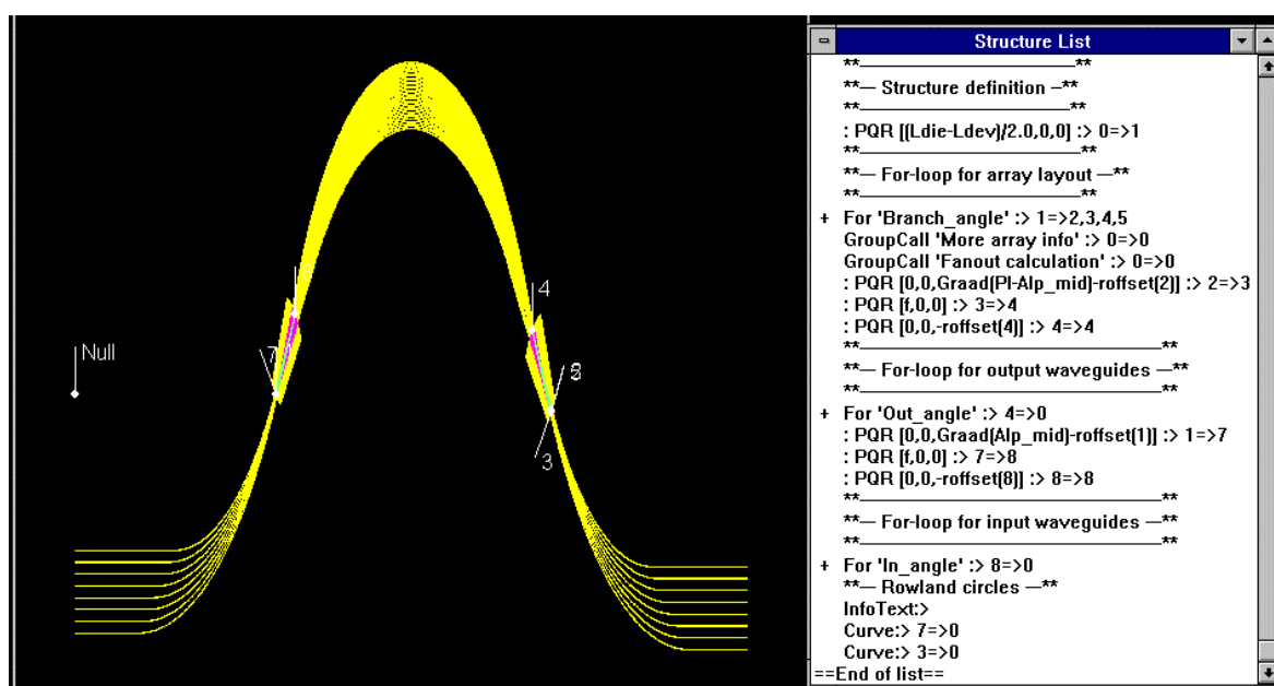
Figure 12. Total layout of the AWG and corresponding section of the 'Structure list'
