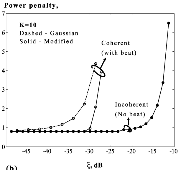
Fig. 6. Power penalty versus (a) K and (b) \xi for coherent and incoherent time-spreading OCDMA networks.
