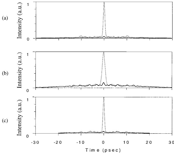
Fig. 9. Intensity autocorrelation data for spectral encoding and decoding separated by fiber, using length-63 M -sequences. Both properly (dashed line) and improperly (solid line) decoded pulses are shown. (a) Only fiber pigtailed (a few meters) separate encoder and decoder. (b) 2.5 km dispersion-compensated links, without phase trimming by LCM. (c) 2.5 km dispersion-compensated link, with phase trimming by LCM.
