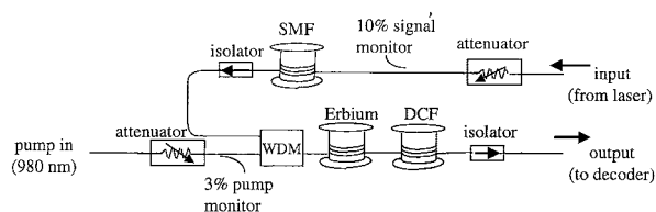
Fig. 3. Chirped pulse amplification erbium doped fiber amplifier.
