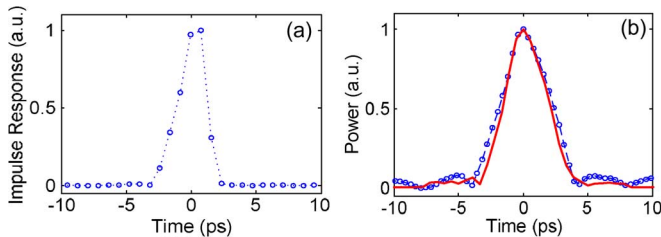
Fig. 4. Experimental results. (a) Measured system impulse response. (b) Synthesized triangular waveforms obtained from the measured LCFBG spectral response (circle line) and from the measured phase response with ideal amplitude response (solid line).
