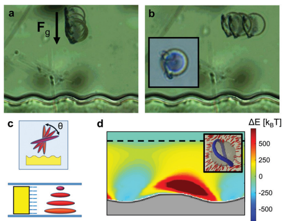
Fig. 5 Homeotropic particle with a twisted loop defect in 75^\circ -twisted cholesteric liquid crystals in a vessel with strong planar anchoring. (a) Time-stack visualization (frame rate: 1 image per min) of the trajectory of a particle under the effect of an external driving force F_g . The particle stops at an equilibrium site determined by the balance between driving and elastic forces. (b) Time-stack visualization (frame rate: 1 image per min) of the same particle in (a) after approach. The particle is able to move because of diffusion and internal drift (no pinning at the boundary), but keeping the same distance from the wall. Inset: Snapshot of the particle under crossed-polarizers, showing the twisted loop. (c) Schematic of the experimental setup. Top view (top) shows the twist of the director field by an angle \theta along the vertical axis. Side view (bottom) shows the director field orientation at the homeotropic wall and in the far field. (d) 2-D color map of the energy landscape \Delta E as a function of the particle position. Inset: Twisted loop defect around a particle, resulting from numerical simulations.
