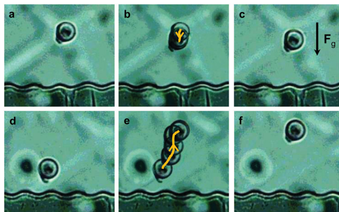
Fig. 4 Particles with a curled dipole in 75^\circ -twisted cholesteric liquid crystals. (a–c) Initial state (a), time-stack visualization (frame rate: 1 image per min) of the trajectory (b) and final state (c) of a particle in the far field under the action of a driving force directed toward the wall. The particle approaches the top of the hill up to the equilibrium site in (c), given by the balance of elastic and driving forces, and stays there until the end of the acquisition. (d–f) Initial state (d), time-stack visualization (frame rate: 1 image per min) of the trajectory (e) and final state (f) of a particle starting in close proximity to the wall (no external force involved here). The particle is initially repelled from the wall until the repulsive gradient becomes negligible.
