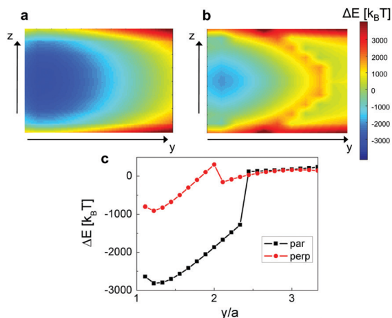
Fig. 7 Numerical simulations of homeotropic colloids wound by twisted loop defects in the \pi -twisted cell. (a) 2-D map of a particle centered on the dale as a function of the vertical position z and distance from the wall y for configuration 1. (b) 2-D map of a particle centered on the dale as a function of the vertical position z and distance from the wall y for configuration 2. (c) Comparison of the energies in the two cases, at fixed height ( z = t/2 ). Particle in parallel configuration (black curve) docks in the dale. Colloid in perpendicular configuration (red curve) is arrested by a barrier around y = 2a .
