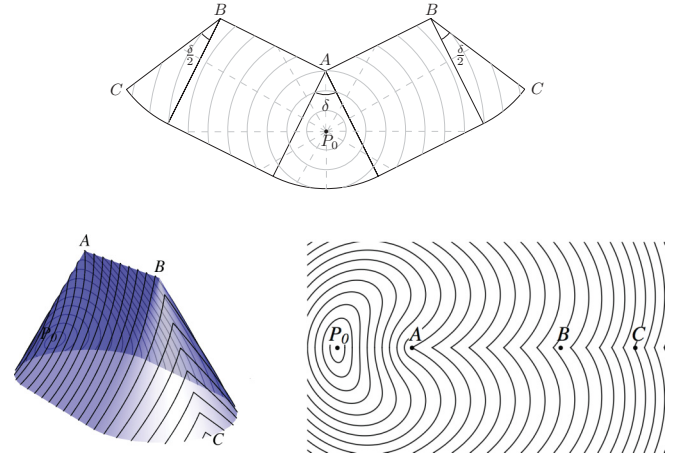
FIG. 7. (Color online) Substrate in the shape of a tent. The top panel shows a flattened model from which a tent can be constructed by gluing along the lines AB and the lines BC . It also shows a point disclination at P_0 and its associated geodesics (dashed lines) and layers (solid lines). The second and third panels show the corresponding layers in the 3D tent and their 2D projection for the case when \delta = \pi and \overline{AB} = \overline{AP_0} = 1 . A , B , and P_0 label the cones apices and the prescribed disclination location, respectively.
