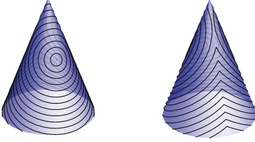
FIG. 4. (Color online) Layer structure on the 3D cone for a deficit angle \delta = 5\pi/4 . The image on the right shows the back of the image on the left and vice versa .
