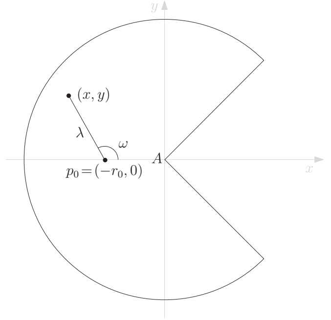
FIG. 3. Cut-disk view of the cone, showing a parametrization of geodesics emanating from a point disclination.
