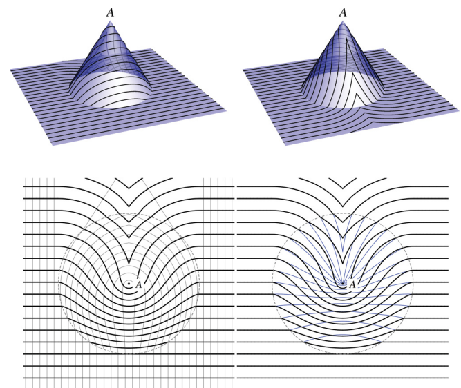
FIG. 9. (Color online) Conical bump with deficit angle given by \pi . We consider as boundary conditions layers parallel to the X axis at Y \rightarrow -\infty . The top panels show the layers on the 3D bump. The bottom left panel shows the projected layers (black) and projected geodesics (gray) on the substrate; notice that they are not orthogonal to each other in the plane metric. The bottom right panel shows the projected layers (black) along with fictitious layers (thin blue lines) which are constructed by demanding orthogonality with the projected geodesics (see text). The intersection between the cone and the plane is depicted by a dashed circle and A labels the cone apex.
