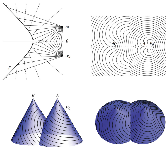
FIG. 8. (Color online) Smectic layers on two intersecting cones with deficit angle \pi and apices A, B . The layer structure is determined by a point disclination at P_0 , located a distance r_0 from apex A as measured on the cone. The horizontal distance between the two apices is chosen to be 2r_0 . The top left panel shows geodesics in the flattened out model of the rightmost cone. Notice that the cut line L (Fig. 2) coincides, in this case, with the positive and negative y axes so that (0, r_0) and (0, -r_0) represent the same point. The intersection line is represented by \Gamma . Geodesics on the rightmost cone are represented by solid lines while the mirror reflection of those geodesics that enter the leftmost cone are depicted by dashed lines. The remaining panels show the layer structure on the cones.
