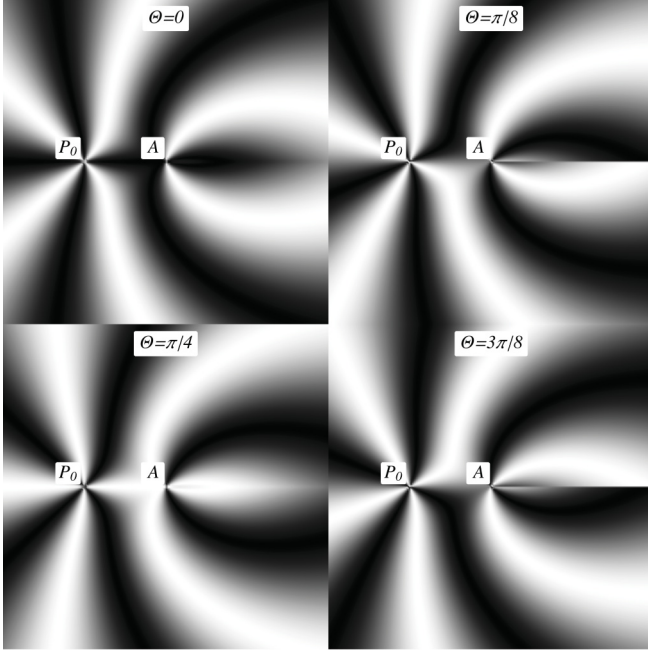
FIG. 6. Schlieren textures for deficit angle \delta = 3\pi/2 , with the polarizer direction at angles of \Theta = 0, \pi/8, \pi/4 , and 3\pi/8 with the X axis, respectively. The analyzer direction rotates to remain perpendicular to the polarizer direction. A and P_0 label the cone apex and the disclination location, respectively.
