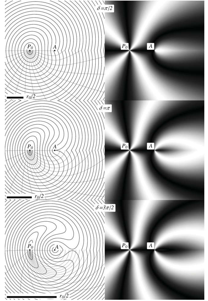
FIG. 5. Left panels show the layer structure (black lines) superimposed on geodesics (gray lines on the bottom half) on the cone, as seen from above (i.e., projected on the XY plane), for deficit angles \delta = \pi/2, \pi , and 3\pi/2 , respectively. The right panels show the corresponding schlieren textures for the same deficit angles. A and P_0 label the cone apex and the disclination location, respectively.
