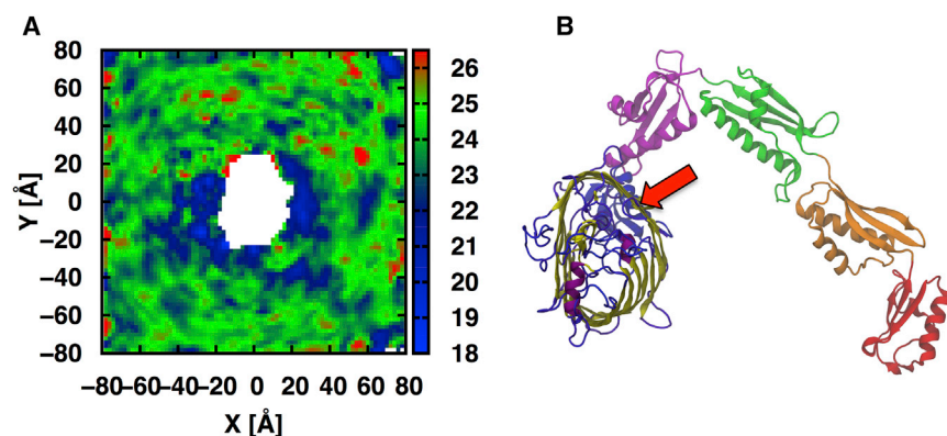
FIGURE 6 (A) Two-dimensional z -thickness of the LPS/phospholipid membrane with embedded full-length BamA. Average of replicas 1–3. Thickness is defined as the distance between the average of C2 and C4 atoms of lipid A (combined) and the average C2 positions of phospholipids within a 2 Å grid and represents the hydrophobic thickness. (B) The relative orientation of the embedded BamA; the red arrow points to the strand 1–16 seam position. The z -thickness of individual replicas is shown in Fig. S11. To see this figure in color, go online.
